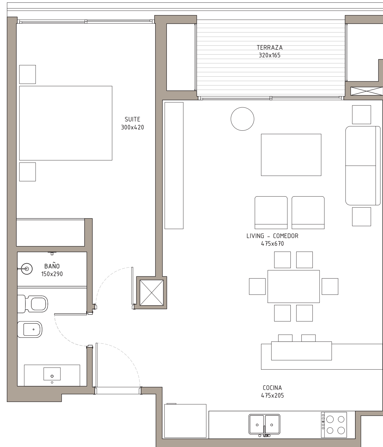
1D Escala 1:50
